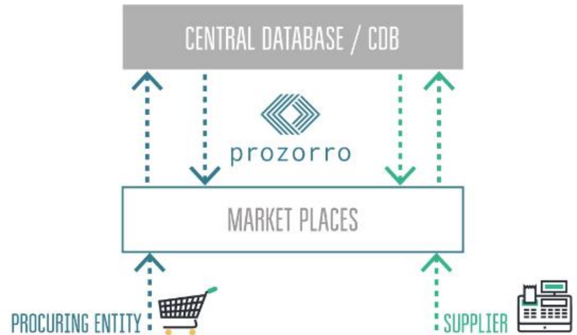
The Hybrid Architecture of ProZorro
